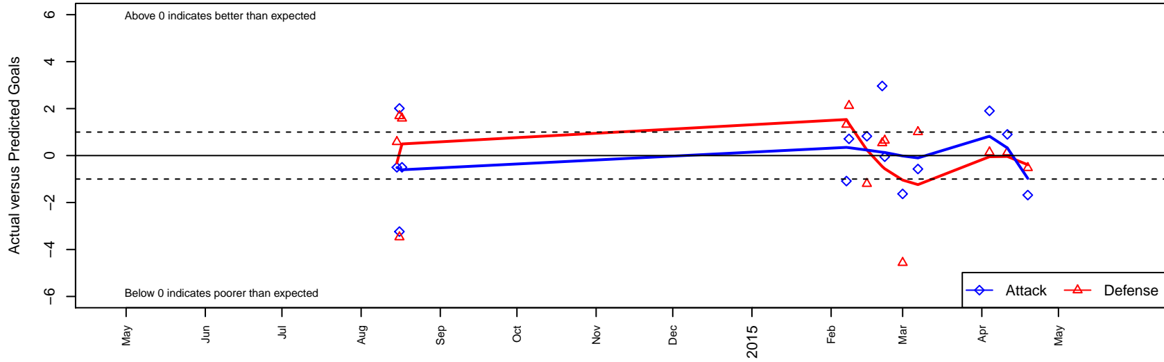
Salem Chelsea B03 Dots are actual minus expected GF (blue circles) and GA (red triangles). Blue line is smoothed change in attack strength. Red is smoothed change in defense strength.
